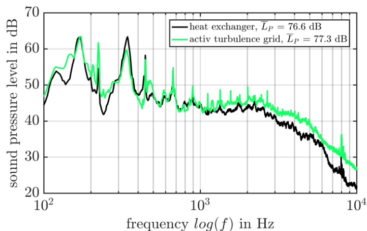
Figure 6: Sound pressure spectra of the heat exchanger ( Tu_{glo} = 8.12\% , \lambda = 8.34 mm) and the active turbulence grid ( Tu_{glo} = 8.15\% , \lambda = 10.48 mm) at the design point ( \dot{V} = 1.4 m 3 /s).
