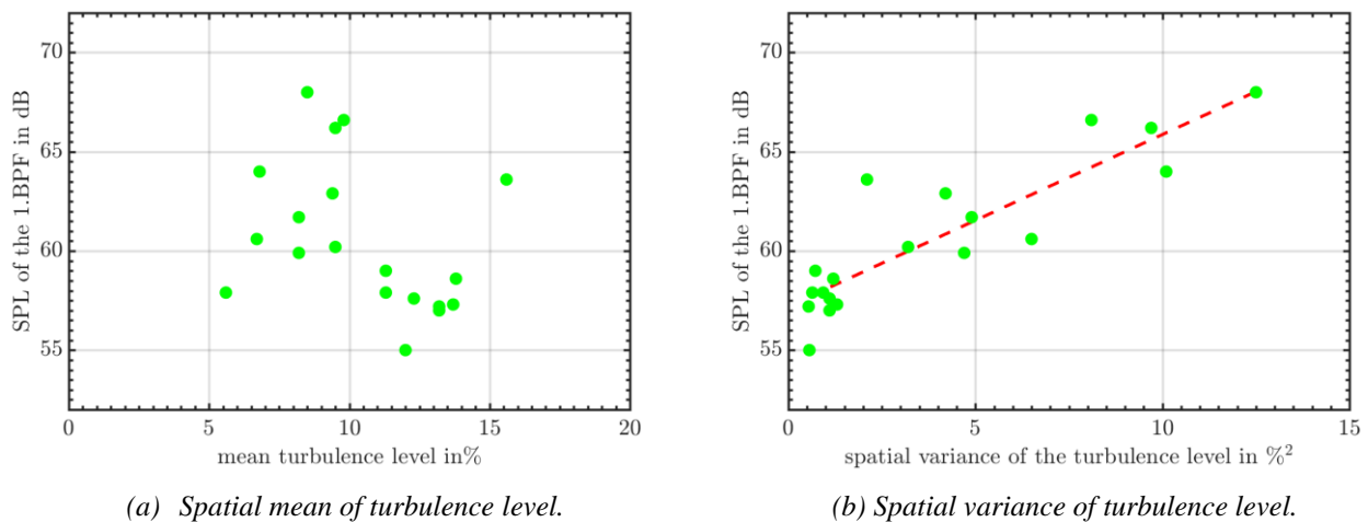
Figure 7: Influence of the spatial mean of the turbulence level and the spatial variance of the turbulence level on the sound radiation of the axial fan at the first blade passing frequency (1.BPF).
