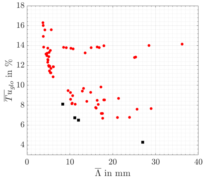
Figure 4: Characteristic map of the induced turbulence characteristics of heat exchangers (■) and different active turbulence grid modes(●).
