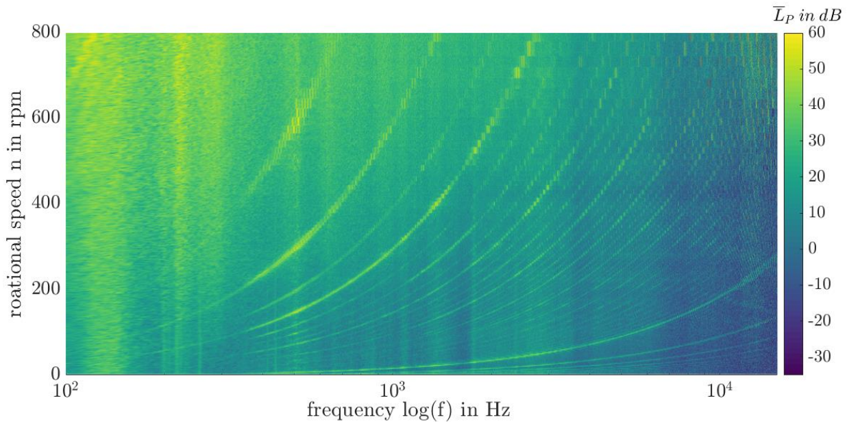
Figure 3: Campbell-plot of the self-induced noise of the active turbulence grid.
