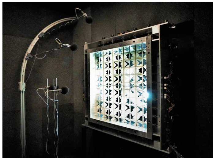
Figure 2: Active turbulence grid inside the anechoic chamber.
