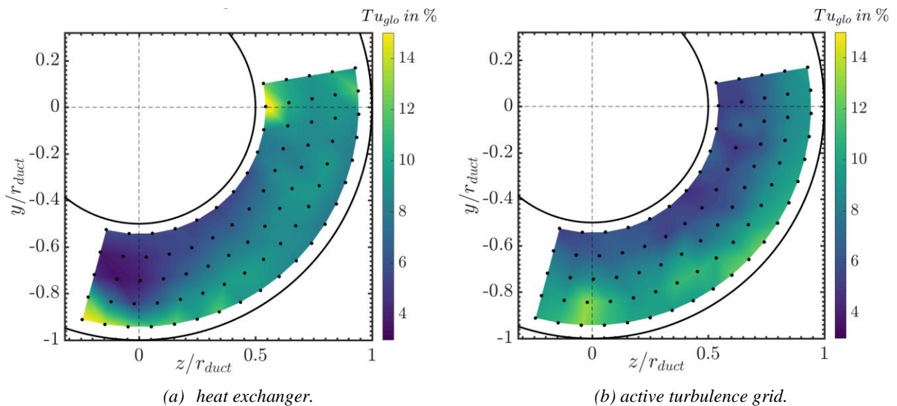
Figure 5: Comparison of field of turbulence level between heat exchanger and imitated flow field by active turbulence grid ( \dot{V} = 1.4\text{ m}^3/\text{s} ).
