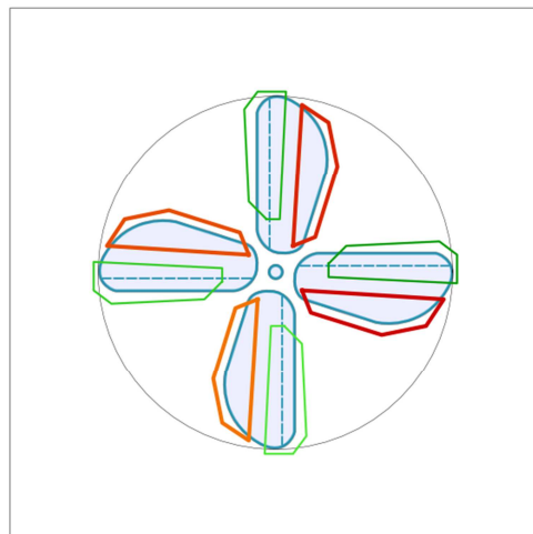
Figure 3: Schematic of the fan with assigned integration sectors. Shades of red: leading edges, shades of green: trailing edges.
