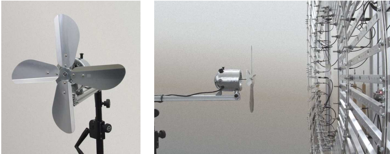
Figure 1: Fan used for the measurements. Fan with microphone array (only the inner ring of microphones was used).
