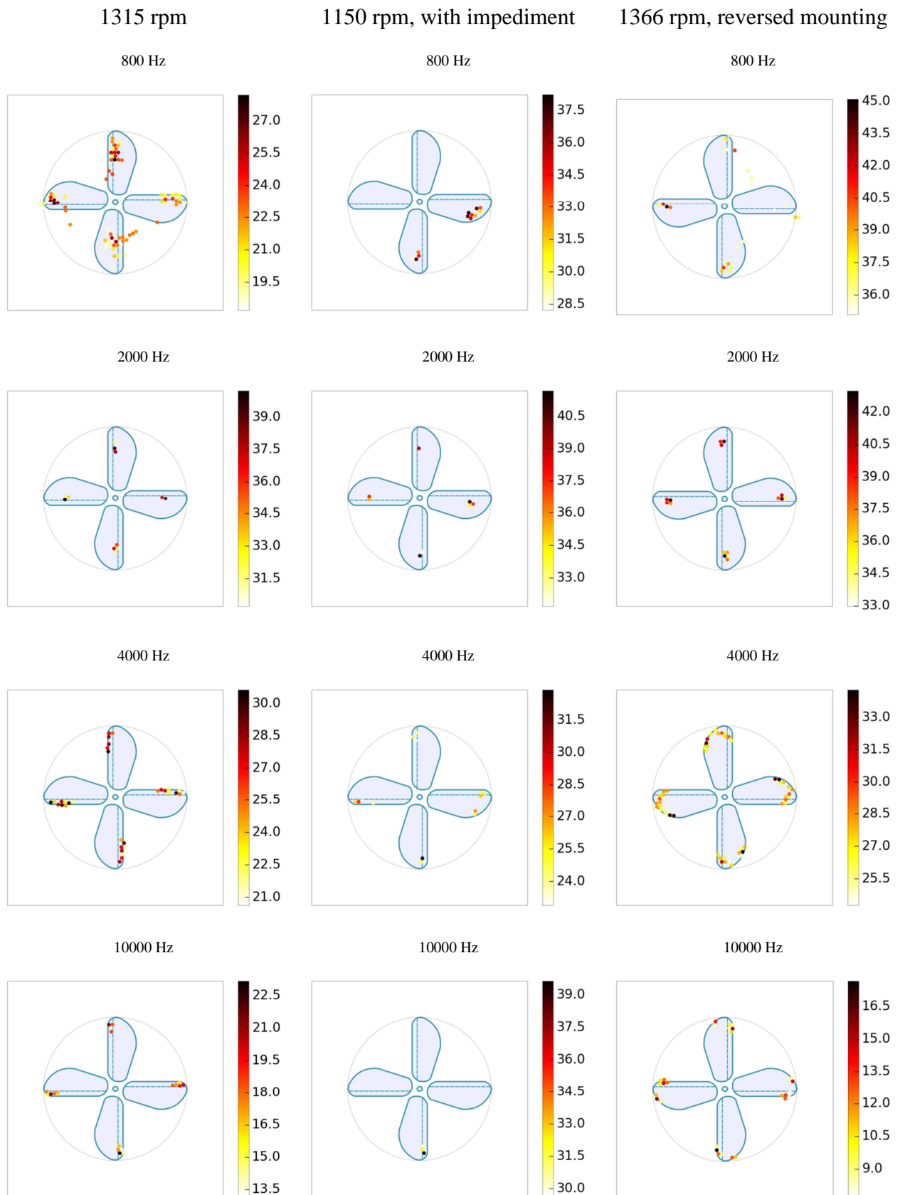
Figure 3: CLEAN-SC sound maps for a clock-wise rotating fan using the virtual rotating array method. The results of three different measurement cases (columns) are evaluated at exemplary third-octave bands (rows), all values in dB.
