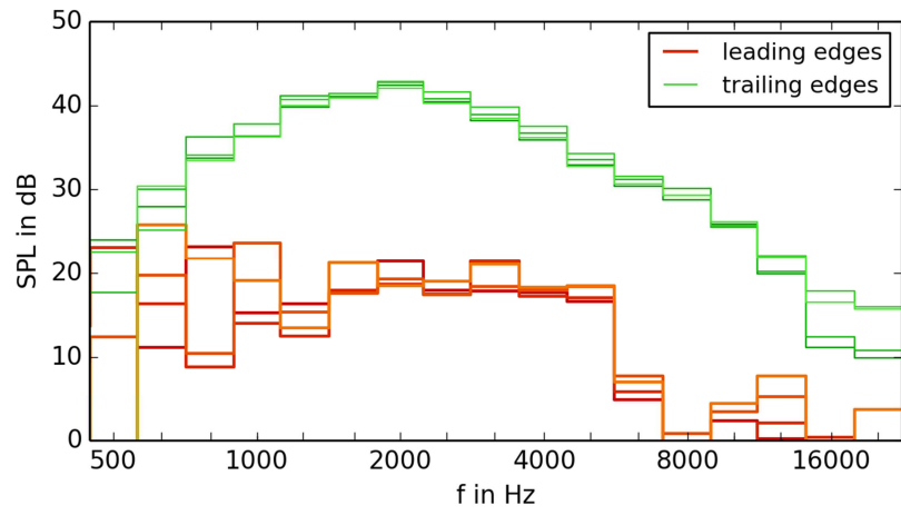
Figure 5: Leading and trailing edge spectra for the fan at 1315 rpm.
