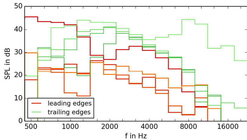
Figure 6: Leading and trailing edge spectra for the fan with applied impeding body at 1150 rpm.
