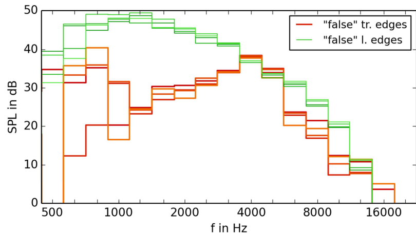
Figure 7: Leading and trailing edge spectra for the backwards mounted fan at 1366 rpm.
